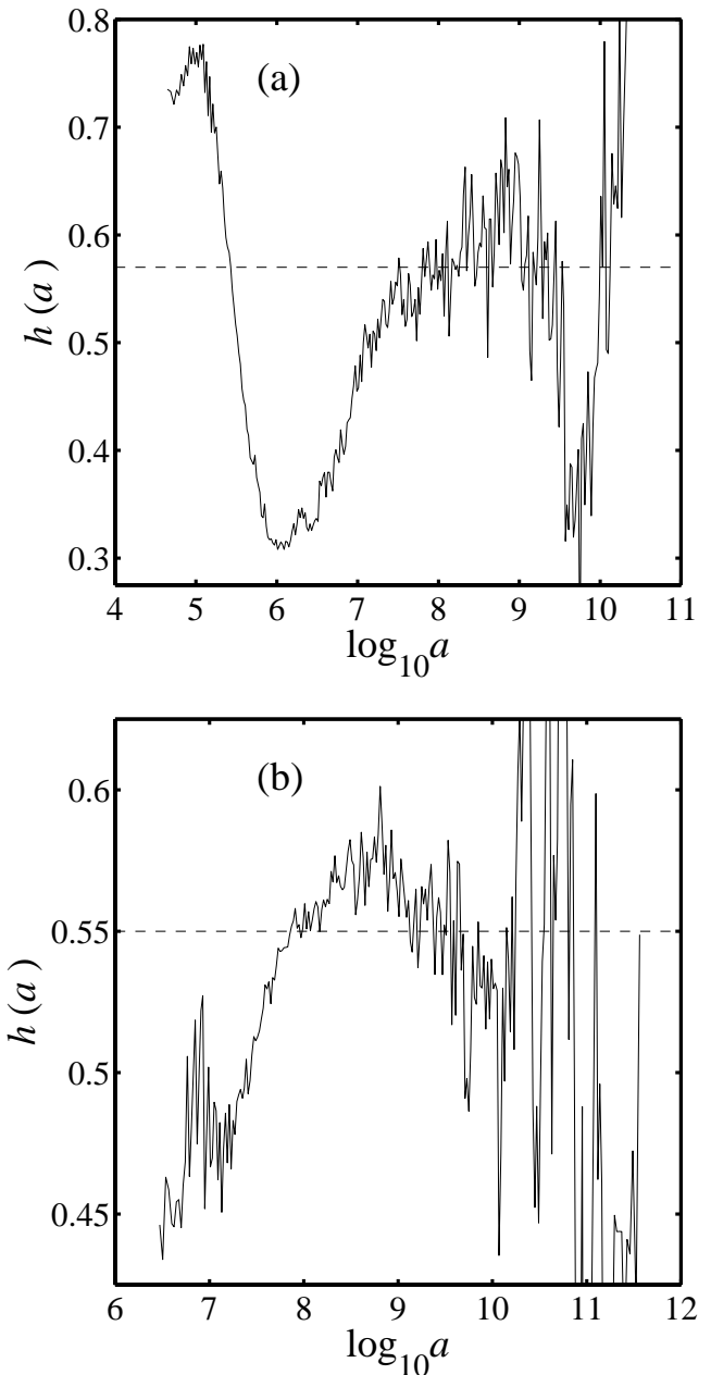
FIG. 9: Variation in Hack’s exponent for the Kansas, (a), and the Mississippi, (b). The area a is in \text{m}^2 . The plots are derivatives of the mean-Hack distributions given in Figures 6(a) and 6(b). Both derivatives have been smoothed by taking running averages over 0.64 orders of magnitude in a . For the Kansas, the dashed line is set at h = 0.57 , Hack’s exponent estimated via simple regression analysis for points with 10^7 < a < 10^{10} \text{m}^2 . The local exponent is seen to gradually rise through the h = 0.57 level indicating scaling is not robust. For the Mississippi in (b), the dashed line is a Hack exponent of 0.55 calculated from regression on data in the interval 10^9 < a < 10^{11.5} \text{m}^2 . The local Hack exponent is seen to gradually rise and fall about this value.
