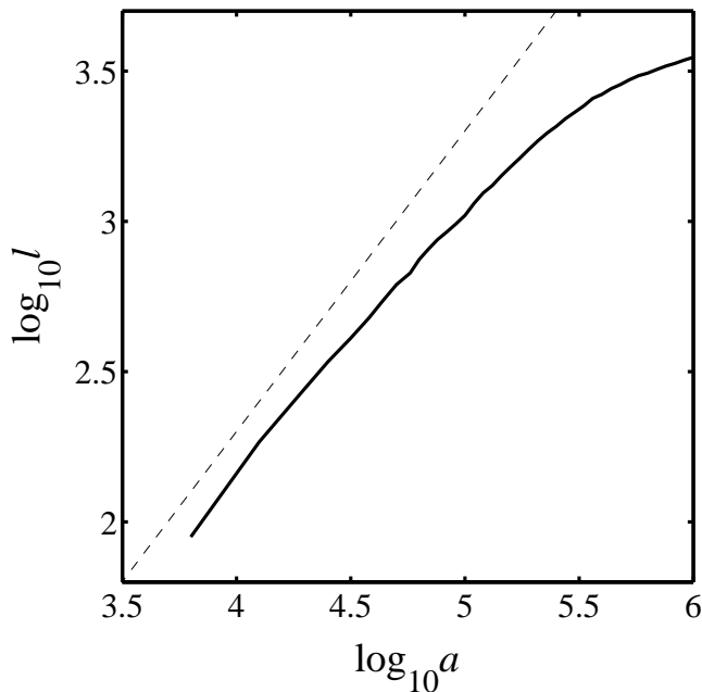
FIG. 7: The linearity of Hack’s law at small scales for the Kansas river. Dimensions are as per Figure 6. The linear regime enters a crossover region after almost 1.5 orders of magnitude in area. This is an expanded detail of the mean Hack’s law given in Figure 6(a) and areas and lengths are in square meters and meters.
