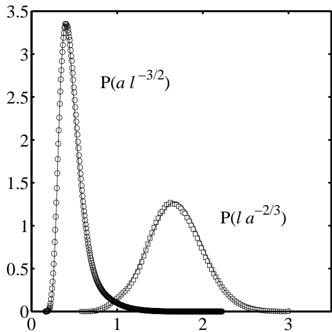
FIG. 3: Cross-Sectional scaling functions of the Hack distribution for the Scheidegger model with lattice constant equal to unity. Both distributions are normalized and all quantities are dimensionless. The right distribution is for l fixed and a varying and is postulated to be a normal distribution. The left distribution for a fixed and l varying and is a form of an inverse Gaussian [58]. The data used was obtained for all sites with l \geq 100 and a \geq 500 respectively. Each distribution was obtained from ten realizations of the Scheidegger model on a 10^4 \times 10^4 lattice.
