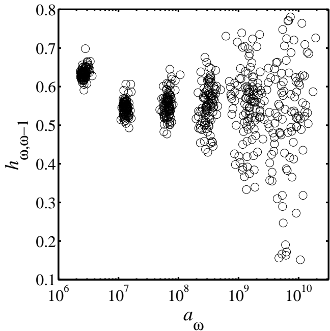
FIG. 11: Differences of the stream order-based version of Hack's law for 104 order \Omega = 7 basins of the Mississippi (compare the continuous versions given in Figure 9). The units of area is square meters and the exponent h_{\omega, \omega-1} is dimensionless. The plots are overlaid to give a sense of the increase in fluctuations of the local Hack exponent h_{\omega, \omega-1} with increasing order \omega . The clusters correspond to \omega = 1, 2, \dots, 7 , moving across from left to right.
