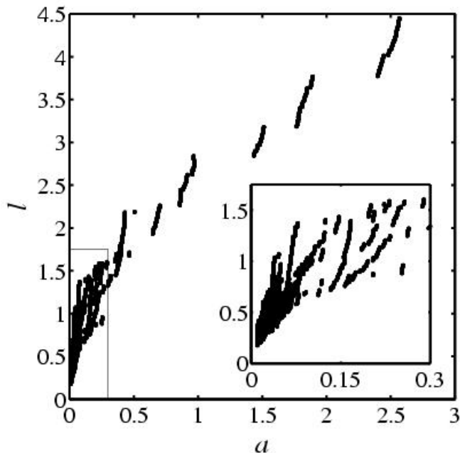
FIG. 10: Hack distribution for the Mississippi plotted in linear space. Area a is given in units of 10^{12} m 2 and length l in 10^6 m. The discreteness of the basin structure is clearly indicated by the isolated, linear fragments. The inset is a blow-up of the box on the main graph.
