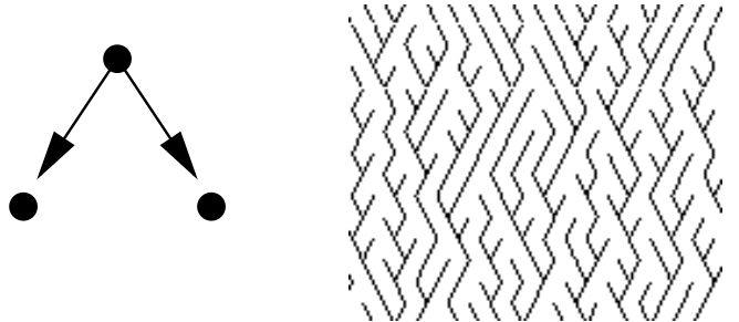
FIG. 2: Scheidegger's model of random, directed networks. Flow is down the page and at each site, stream flow is randomly chosen to be in one of the two downward diagonals. Stream paths and basin boundaries are thus discrete random walks.
