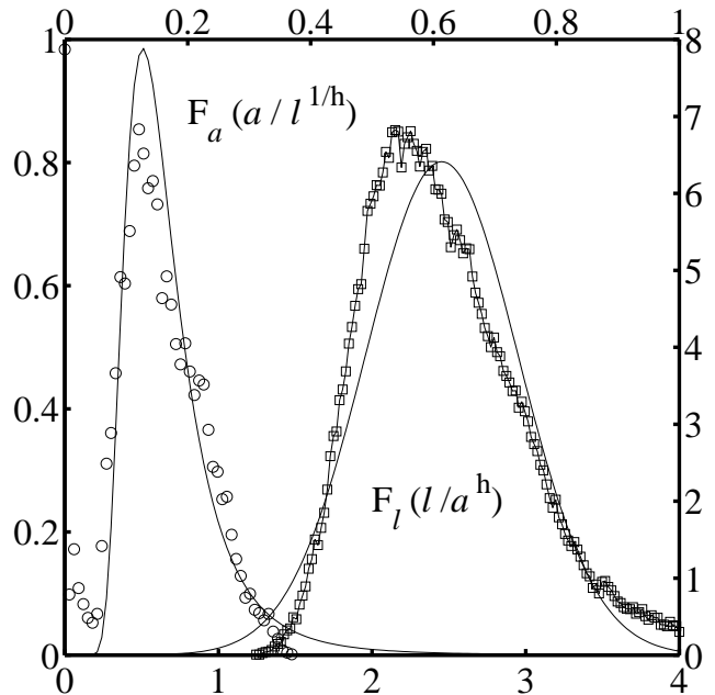
FIG. 5: Cross-sectional scaling functions of the Hack distribution for the Nile. Dimensions are as per Figure 4. The top and right axes correspond to F_a and the bottom and left to F_l . The Hack exponent used is h = 0.50 and the values of the Hack mean coefficient and standard deviation coefficient are estimate to be \theta \simeq 2.45 and \eta \simeq 0.50 [59].
