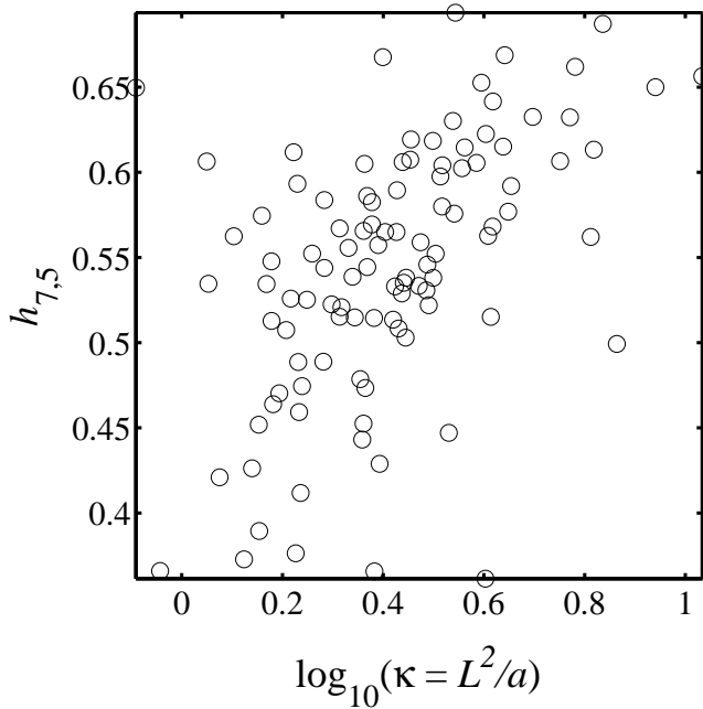
FIG. 13: Correlation between trends in Hack's law and the aspect ratio of a basin as estimated by the dimensionless quantity \kappa = L^2/a . The data is for the order \Omega = 7 basins of the Mississippi and the specific trend is h_{7,5} . The correlation measurements give r = 0.50 , r_s = 0.53 and p_s < 10^{-8} .
