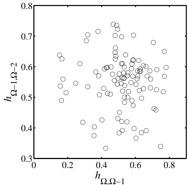
FIG. 12: A comparison of the stream order Hack derivatives h_{\Omega, \Omega-1} and h_{\Omega-1, \Omega-2} for each of the 104 order \Omega = 7 basins of the Mississippi. Both axes are dimensionless. The linear correlation coefficient is r = -0.06 and the Spearman correlation coefficient is r_s = -0.08 . The latter has probability p_s = 0.43 indicating there are no significant correlations.
