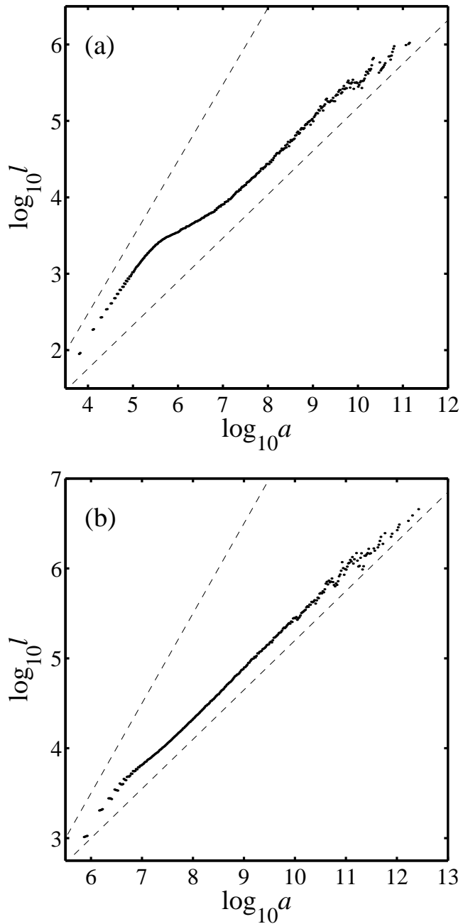
FIG. 6: The mean version of Hack's law for the Kansas, (a), and the Mississippi, (b). The units of lengths and areas are meters and square meters. These are calculated from the full Hack distributions shown in Figures 1(a) and 1(b) by finding \langle l \rangle for each value of basin area a . Area samples are taken every 0.02 orders of magnitude in logarithmic space. The upper dashed lines represent a slope of unity in both plots and the lower lines the Hack exponents 0.57 and 0.55 for the Kansas and Mississippi respectively. For the Kansas, there is a clear deviation for small area which rolls over into a region of very slowly changing derivative before breaking up at large scales. Deviations from scaling are present for the lower resolution dataset of the Mississippi, but to a lesser extent.
