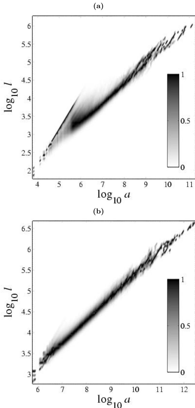
FIG. 1: The Full Hack distribution for the Kansas, (a), and Mississippi, (b), river basins. Area a and length l are in \text{m}^2 and \text{m} respectively. For each value of a , the distribution has been normalized along the l direction by \max_l P(a, l) [49].
