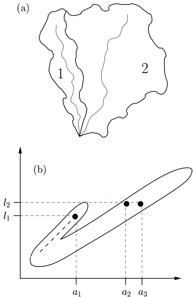
FIG. 8: Origin of the linear branch in the Hack distribution. The sub-basins labeled 1 and 2 depicted in (a) have areas a_1 and a_2 and lengths l_1 and l_2 . These sub-basins combine to form a basin of area a_3 = a_1 + a_2 and main stream length l_3 = \max(l_1, l_2) = l_2 . Since sub-basin 1 is a linear sub-network (a valley) the pair (a_1, l_1) lie along the linear branch of the Hack distribution as shown in (b). Points along the main stream of sub-basin 1 lie along the dashed line leading to the coordinate (a_1, l_1) . On combining with the second basin, the jump in the resultant area creates a jump from (a_1, l_1) to (a_3, l_2) in the main body of the Hack distribution.
