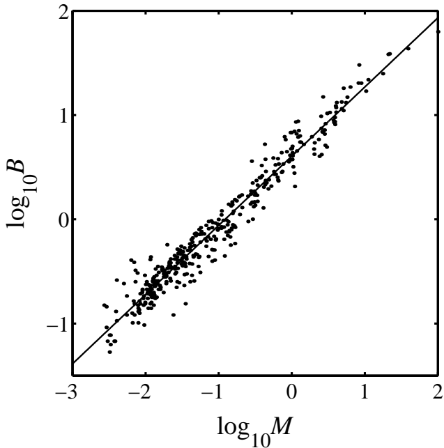
FIG. 2: Metabolic rate, B (watts), as a function of mass, M (kg), for 398 species of birds taken from Bennett and Harvey [30]. The straight line is the result of a regression analysis which gives \hat{\alpha} = 0.664 \pm 0.014 .
