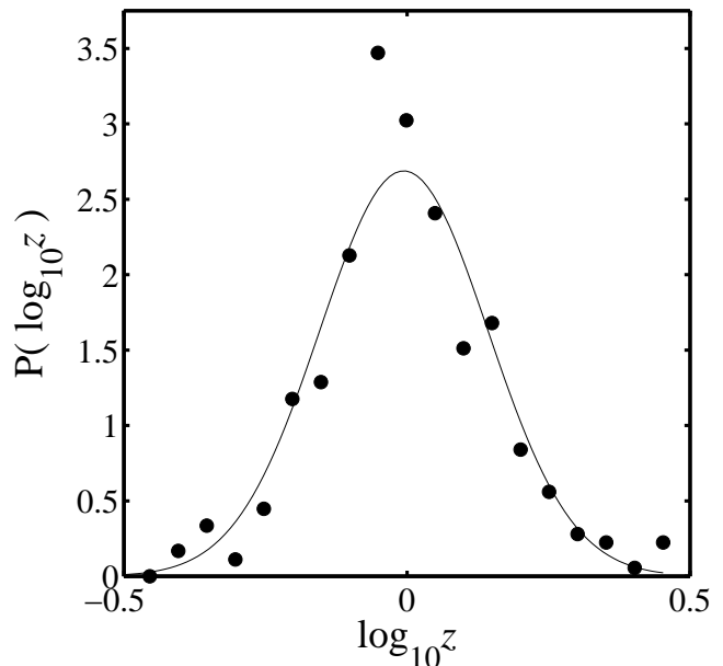
FIG. 3: Fluctuations in metabolic rate for mammals with M \leq 10 kg taken from Heusner’s data set [29]. Here, z = B/cM^\alpha . The scaling function f (see equation (2)) is fitted with a lognormal distribution. Values of B have been renormalized as B/cM^\alpha with \hat{\alpha} = 0.667 and c = 2.58 as explained in the text and partitioned into 20 bins.
