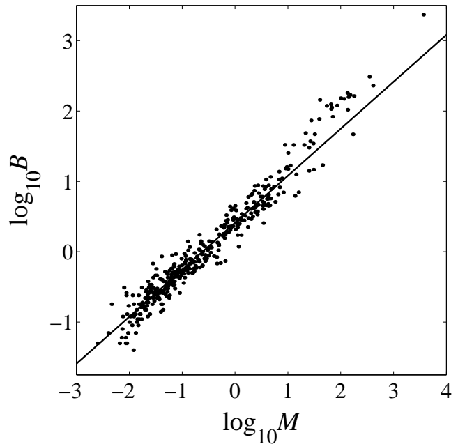
FIG. 1: Metabolic rate, B (watts), as a function of mass, M (kg), for 391 species of mammals. Data taken from Heusner [29]. The straight line represents the best fit for the 357 species with mass less than 10 kg where \hat{\alpha} = 0.668 \pm 0.019 . The upward deviations for species with larger mass (see Table I) may indicate a real biological difference but may also be due to the paucity of data.
