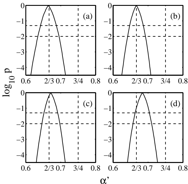
FIG. 4: Test of the null hypothesis H_0 : r_{s,\alpha'}(z_i, M_i) = 0 based on mammalian data from Heusner [29] (see equation (5)). Shown are plots of p(\alpha') for differing mass ranges. In all plots the two dashed horizontal lines correspond to p = 0.05 and p = 0.01 . The individual plots correspond to the following ranges: (a) M < 3.2 kg, (b) M < 10 kg, (c) M < 32 kg, (d) all mammals. For all mass ranges considered, p_{2/3} > 0.05 and p_{3/4} \ll 10^{-4} .
