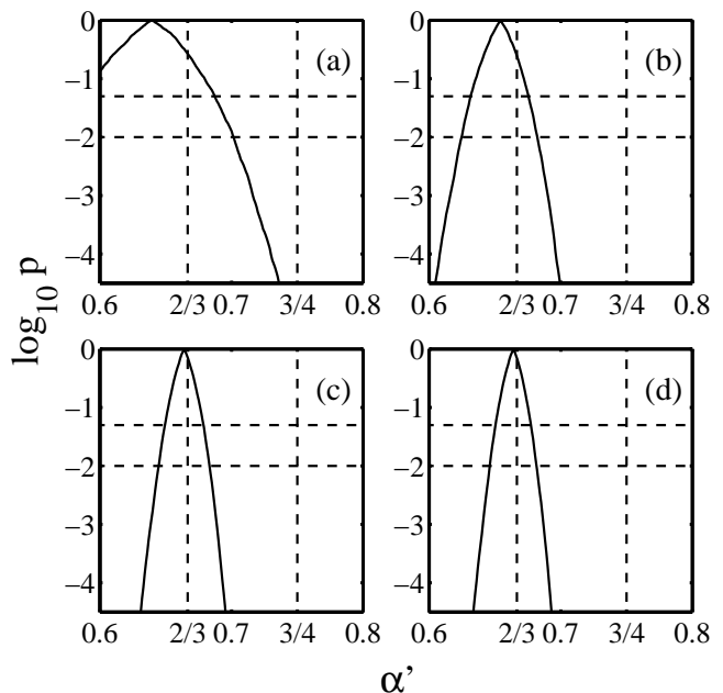
FIG. 5: Test of the null hypothesis H_0 : r_{s,\alpha'}(z_i, M_i) = 0 based on bird data from Bennett and Harvey [30] (see Figure 4 for details). Here, the individual plots correspond to the following ranges: (a) M < 0.1 kg, (b) M < 1 kg, (c) M < 10 kg, (d) all birds. As for the mammal data, p_{2/3} > 0.05 and p_{3/4} \ll 10^{-4} for all mass ranges considered.
