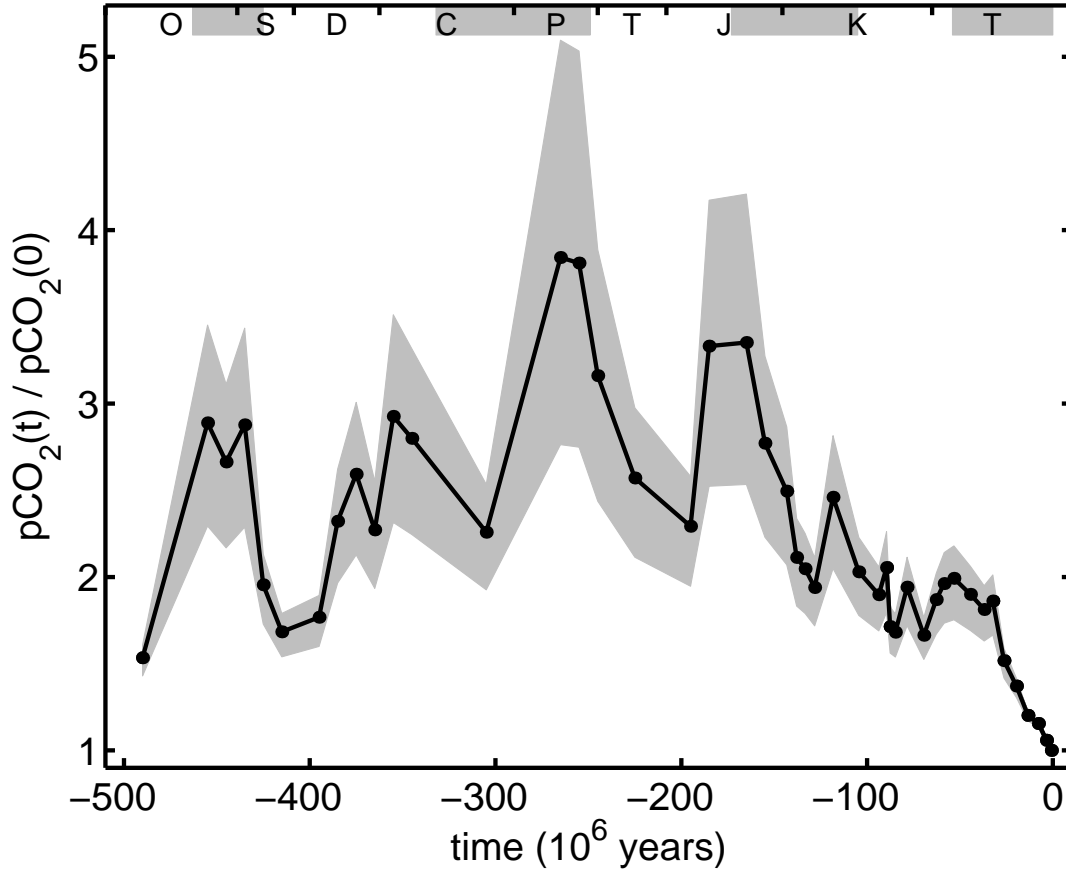
FIG. 4. Fluctuations of p\text{CO}_2 for the last 500 million years, normalized by the estimate of p\text{CO}_2 obtained from the most recent value of \zeta . The solid line is obtained from equation (12) using \varepsilon_0 = 36\% . The lower and upper limits of the gray area surrounding the p\text{CO}_2 curve result from \varepsilon_0 = 38\% and 35\% , respectively. The gray bars at the top correspond to periods when the Earth's climate was relatively cool; the white spaces between them correspond to warm modes [18].
